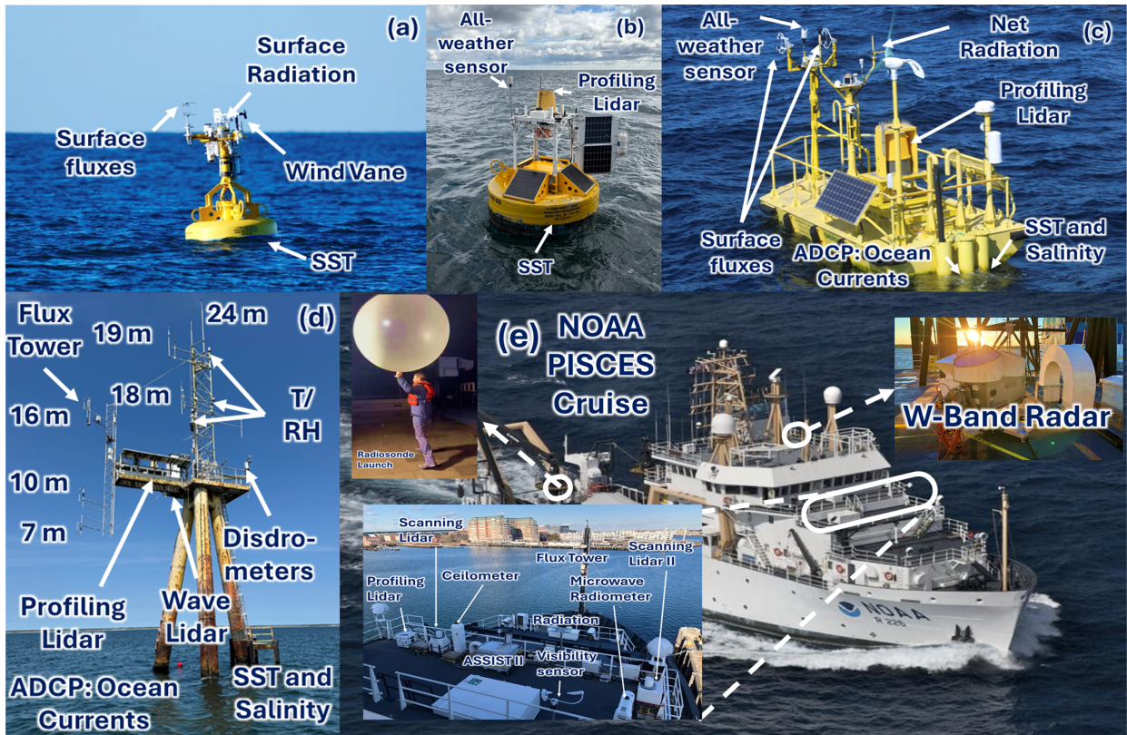
FIG. 5. WFIP3 offshore platforms and buoy systems, including (a) WHOI sentinel surface buoy, (b) WHOI lidar buoy, (c) DOE lidar buoy, (d) WHOI Air-Sea Interaction Tower (ASIT) and (e) NOAA Pisces winter cruise.
